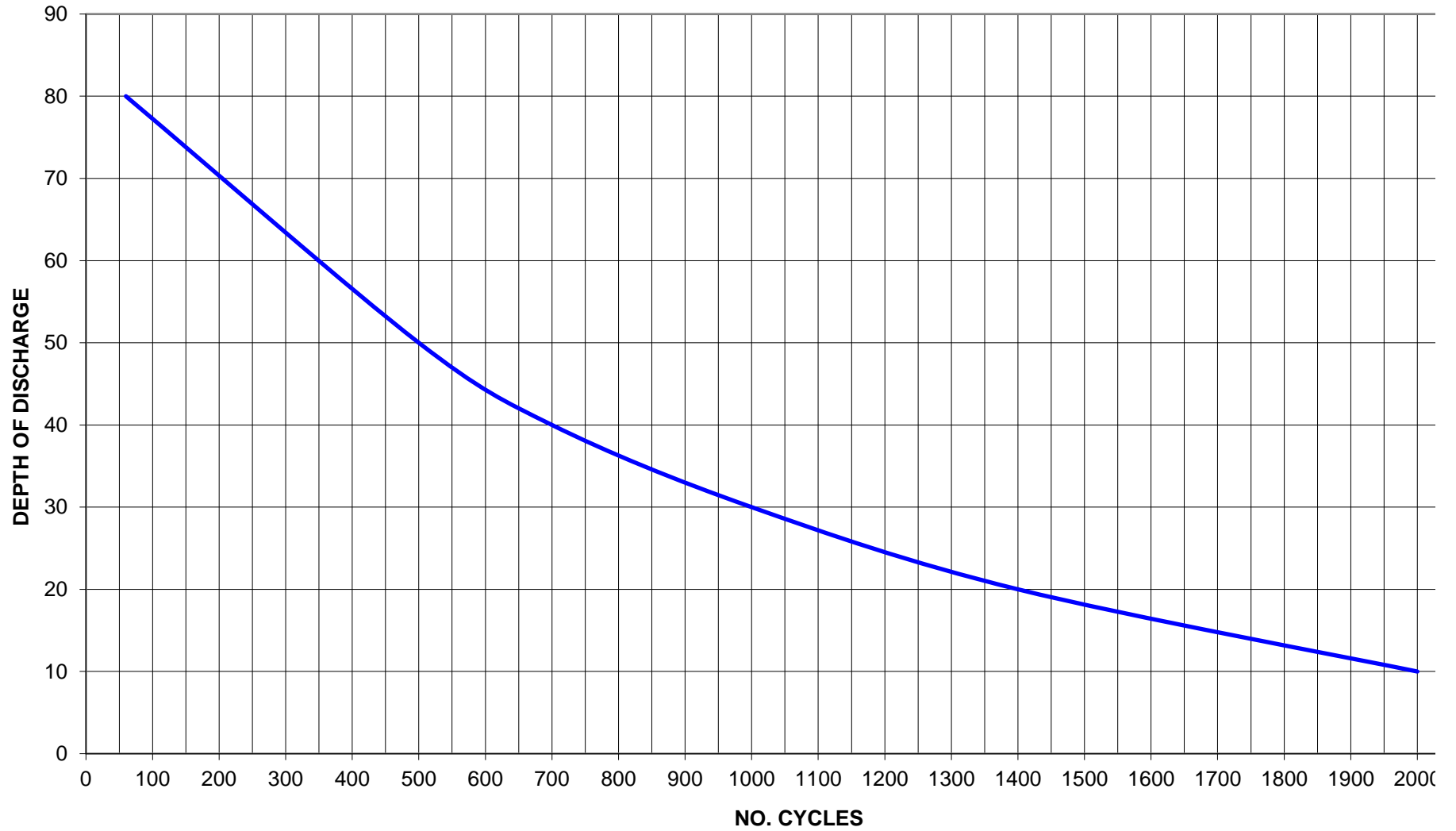
SMF - NO. CYCLES vs DEPTH OF DISCHARGE AT 25°C
